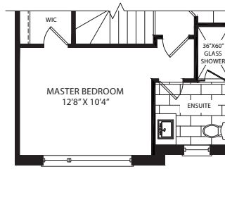
PARTIAL- THIRD FLOOR PLAN ELEVATION 'B'
