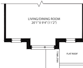
PARTIAL- SECOND FLOOR PLAN ELEVATION 'B'
