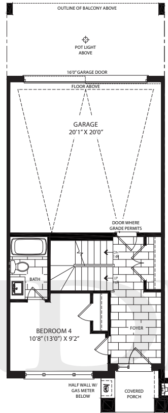
OPT. GROUND FLOOR PLAN 4 BEDROOM W/ BATH ELEVATION 'A'
