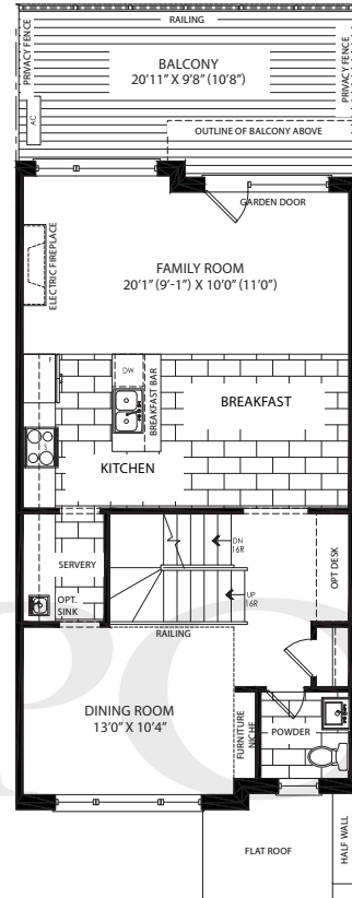
SECOND FLOOR PLAN ELEVATION 'A'
