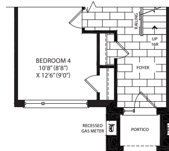
PARTIAL-OPT. GROUND FLOOR PLAN BEDROOM W/ BATH ELEVATION 'B'
