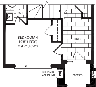
PARTIAL-OPT. GROUND FLOOR PLAN 4 BEDROOM W/ BATH ELEVATION 'B'
