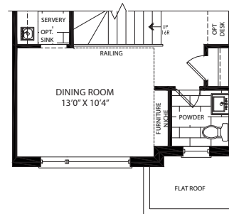
PARTIAL- SECOND FLOOR PLAN ELEVATION 'B'
