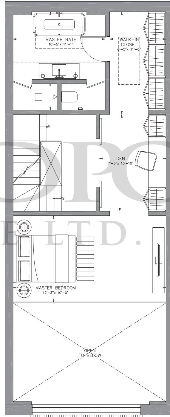
LEVEL 2
