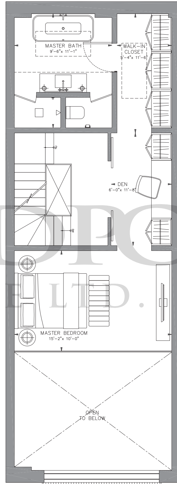
LEVEL 2
