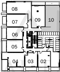
BUILDING OVERVIEW
